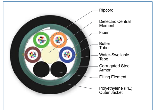
Cross Section of Part Number: 048EUC-T4101D20
