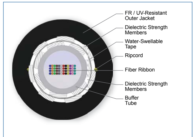
Cross Section of Part Number: 048ECF-14101-20
