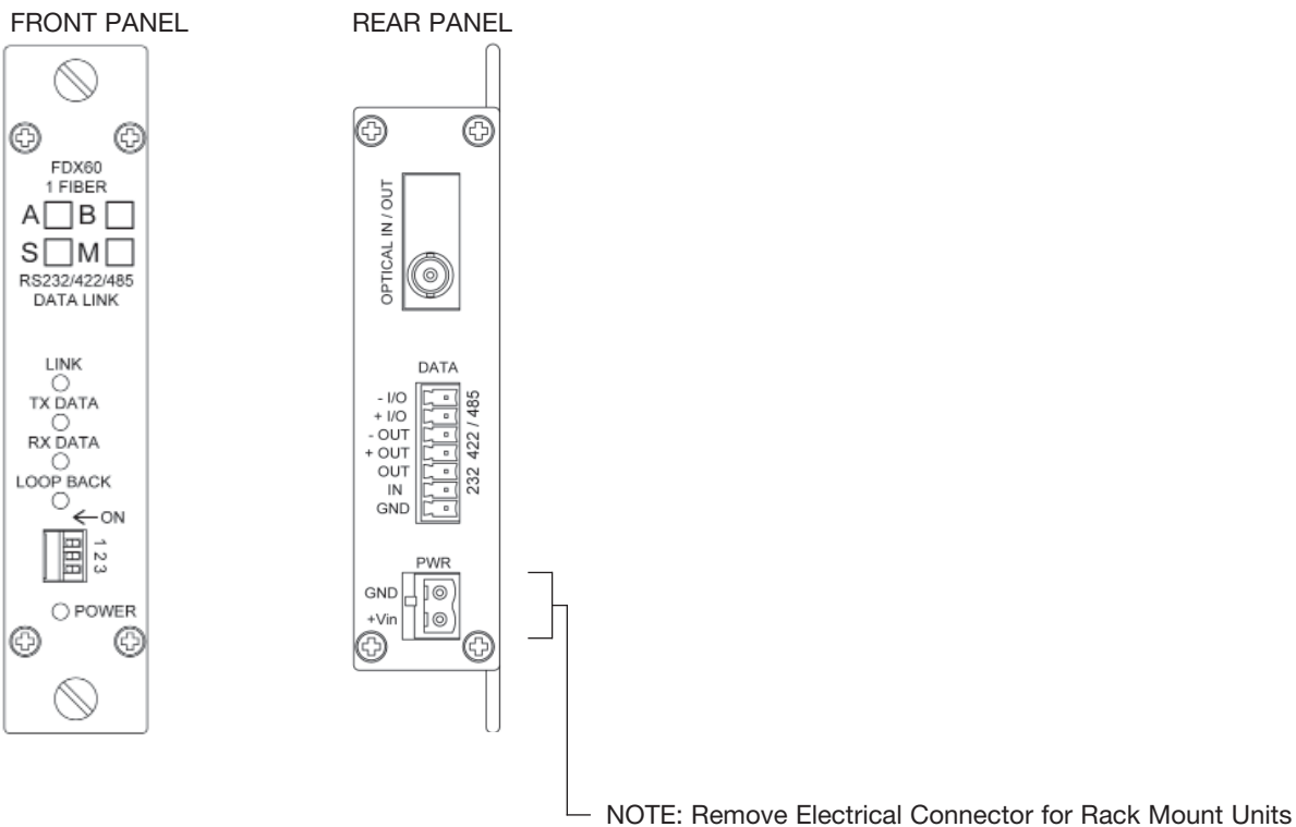
FIGURE 2 – FDX60 1 FIBER TRANSCEIVER
