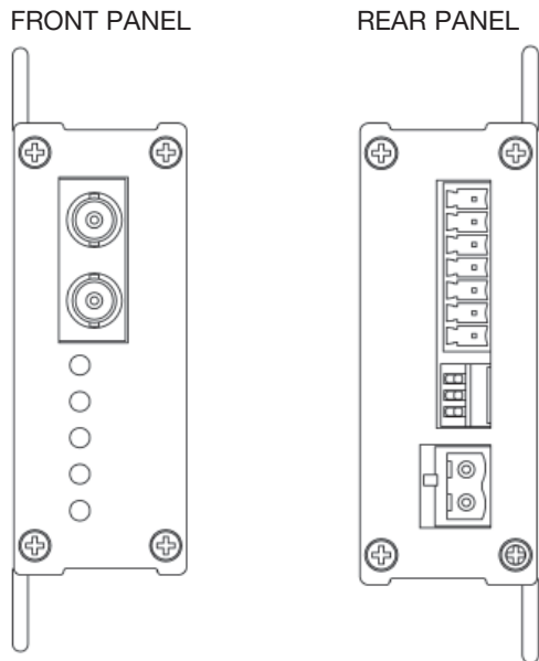
FIGURE 8 – FDX60-M 2 FIBER TRANSCEIVER
