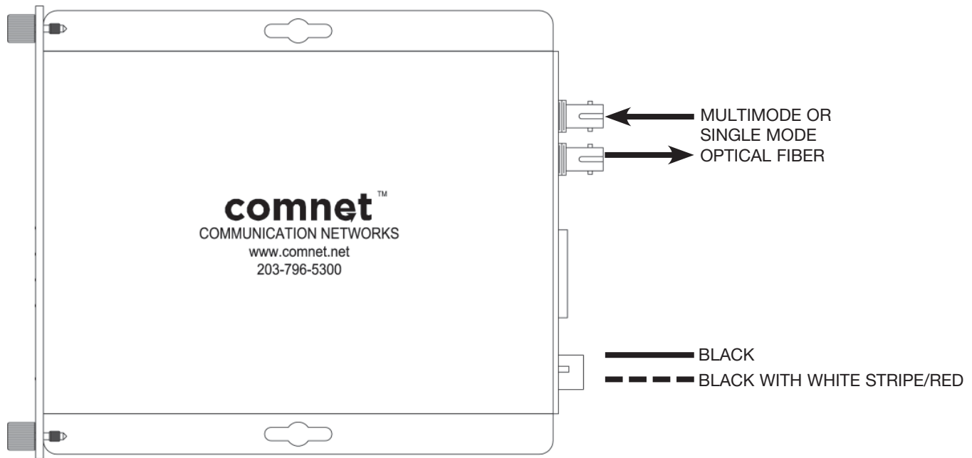
FIGURE 3 – FDX60 2 FIBER TRANSCEIVER
