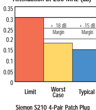
Siemon S210 4-Pair Patch Plug
