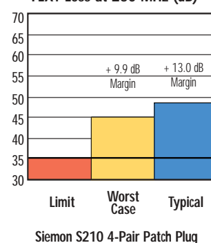
FEXT Loss at 250 MHz (dB)
