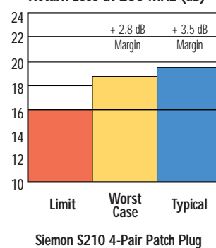
Return Loss at 250 MHz (dB)
