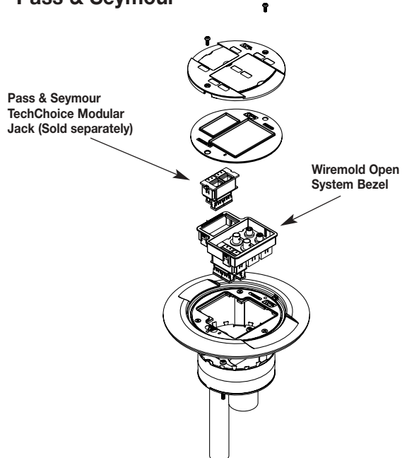
AMD8 Assembled Unit shown with Pass & Seymour Category 5e TechChoice jacks. (Jacks sold separately.)
