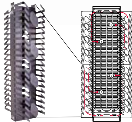
Upper and lower crossover managers with vertical cable managers enable easy, intuitive cable routing.
