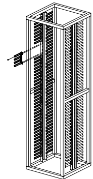
Glide Cable Manager, Cabinet Mount
