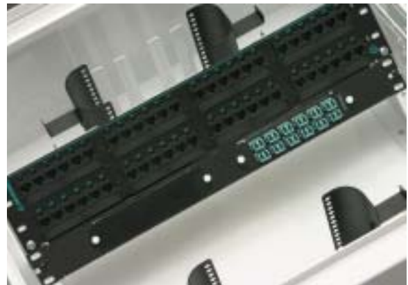
Fiber Zone Box (shown with 48-port copper patch panel and 1U fiber patch panel) | Photo LAN592
