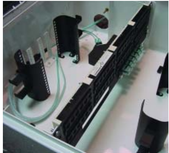
Fiber Zone Box (shown with Plug & Play™ Universal Systems module and copper patch panel) | Photo NS59
